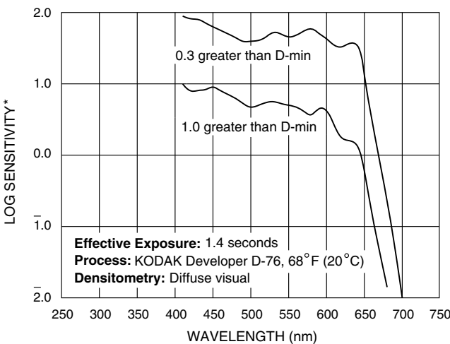
Spectral-Sensitivity Curves*
