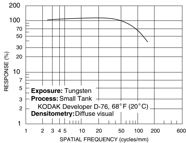
Modulation Transfer Curves
